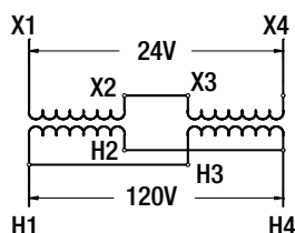
120V TO 24V
