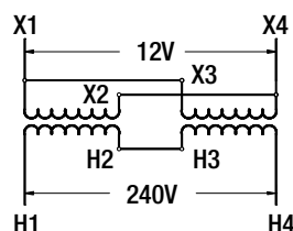
240V TO 12V
