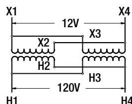
120V TO 12V
