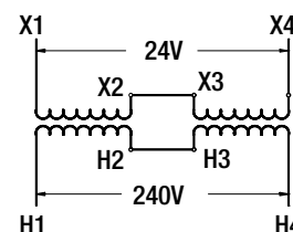
240V TO 24V
